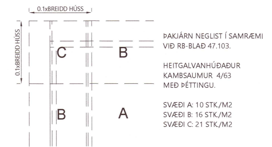
NEGLING ÞAKJÁRNS 1 : 50
