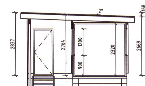
SNID 2-2 1:100
