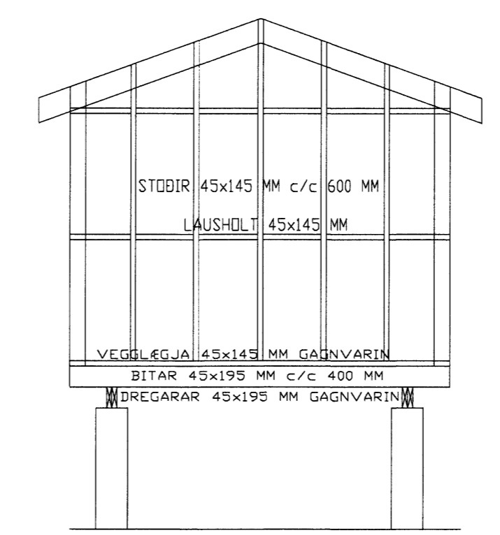
SNID - C 1:50
