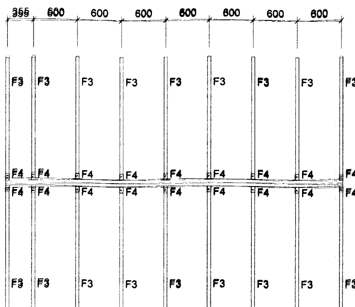
Þakplan mkv: 1:50
