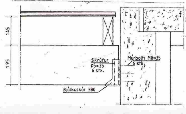
Snid C-C 1:10
