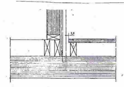
Snid F-F 1:20
