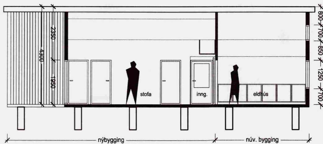
SNID AA
