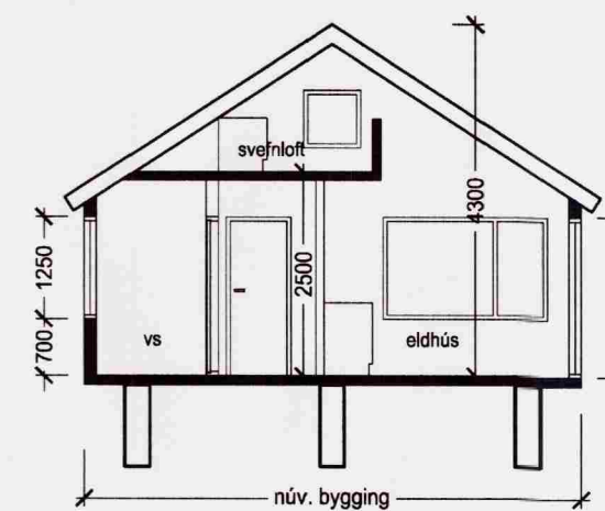
SNID BB
