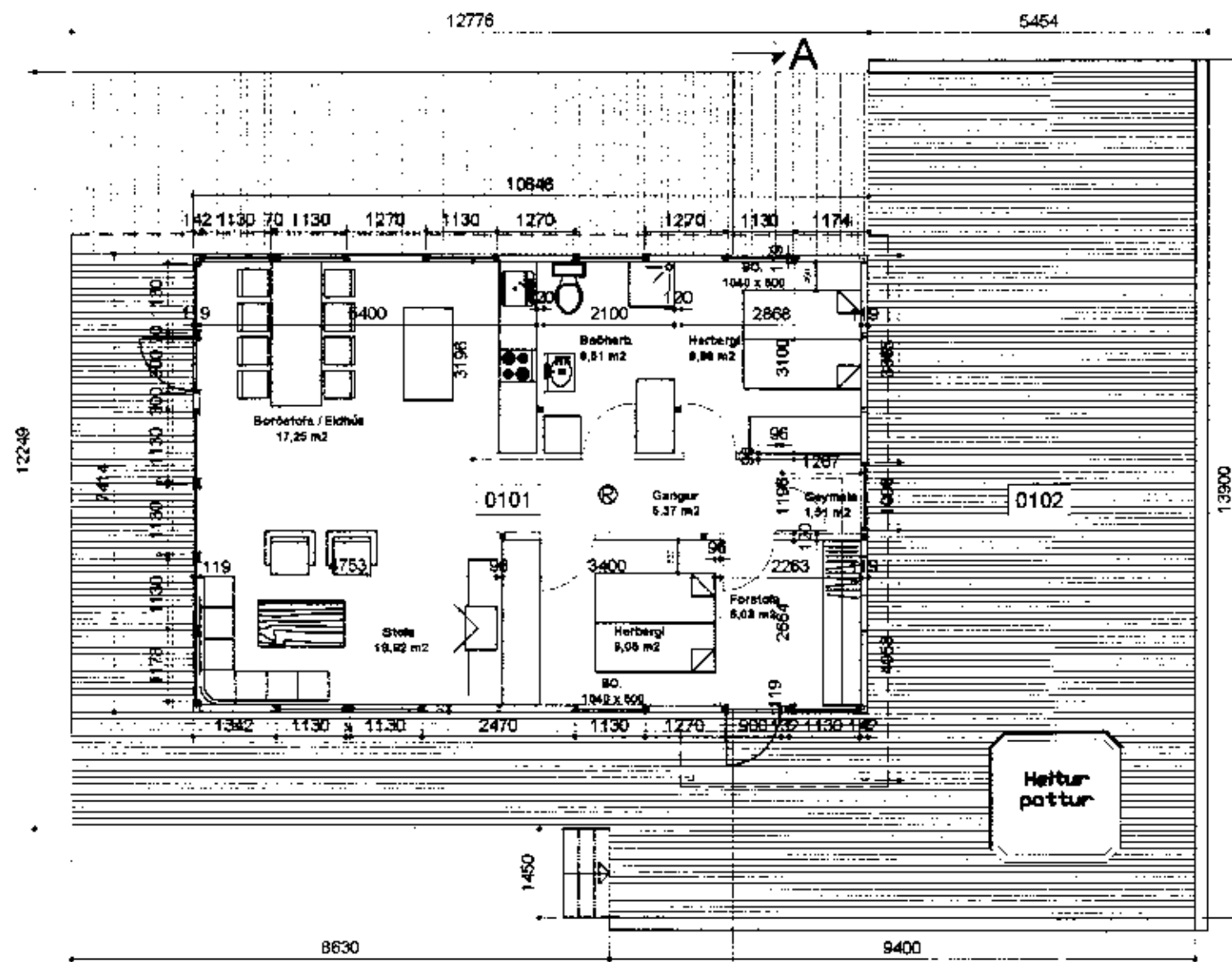
Grunnmynd. m: 1/100.
