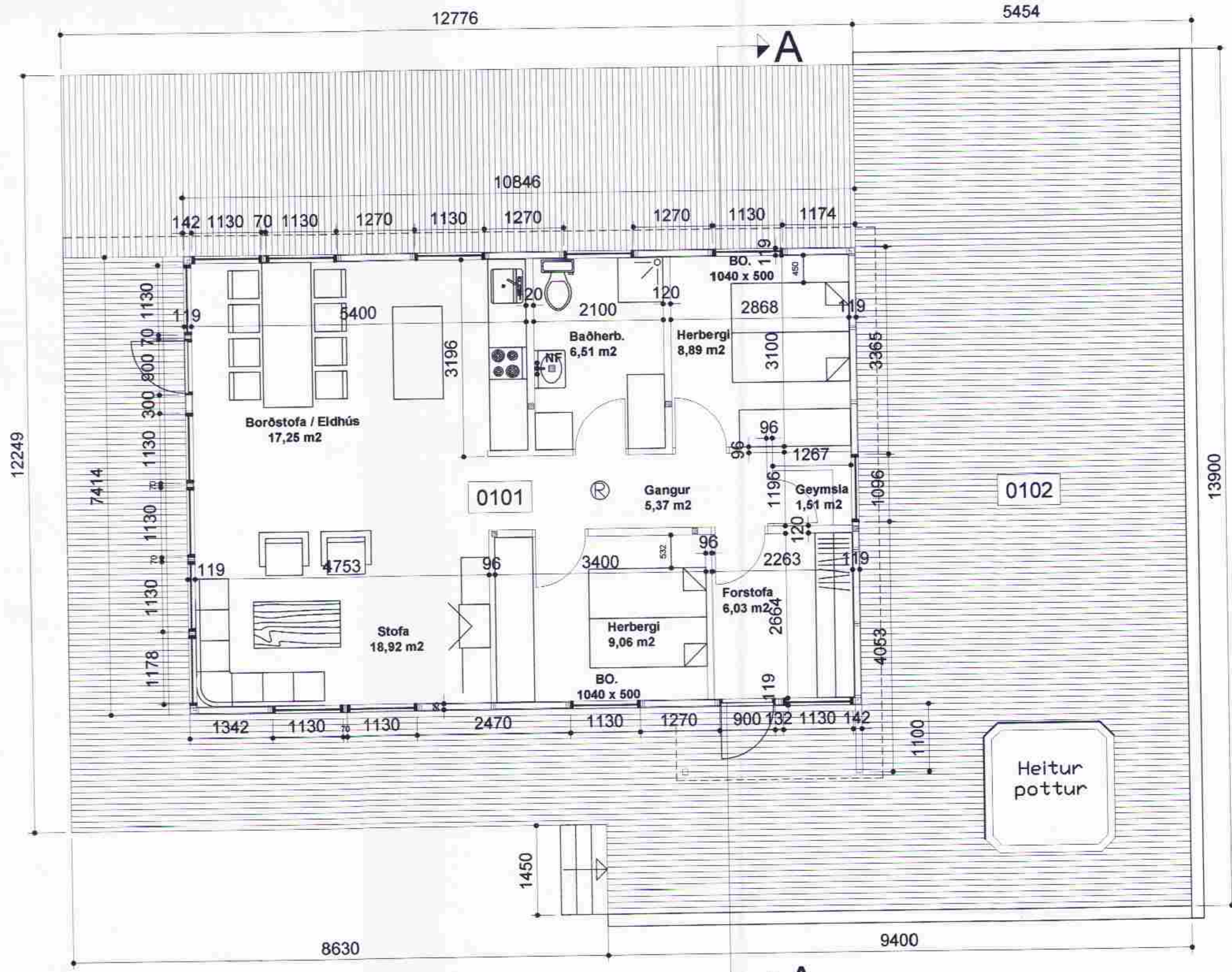
Grunnmynd. m: 1/50.
