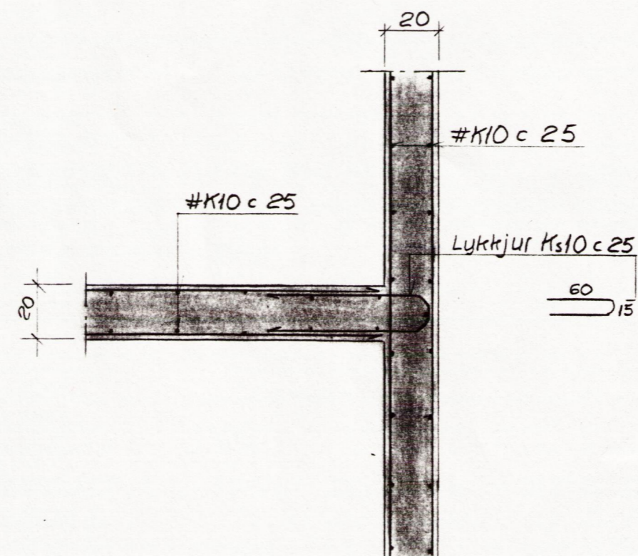
SNID H-H - 1:20
