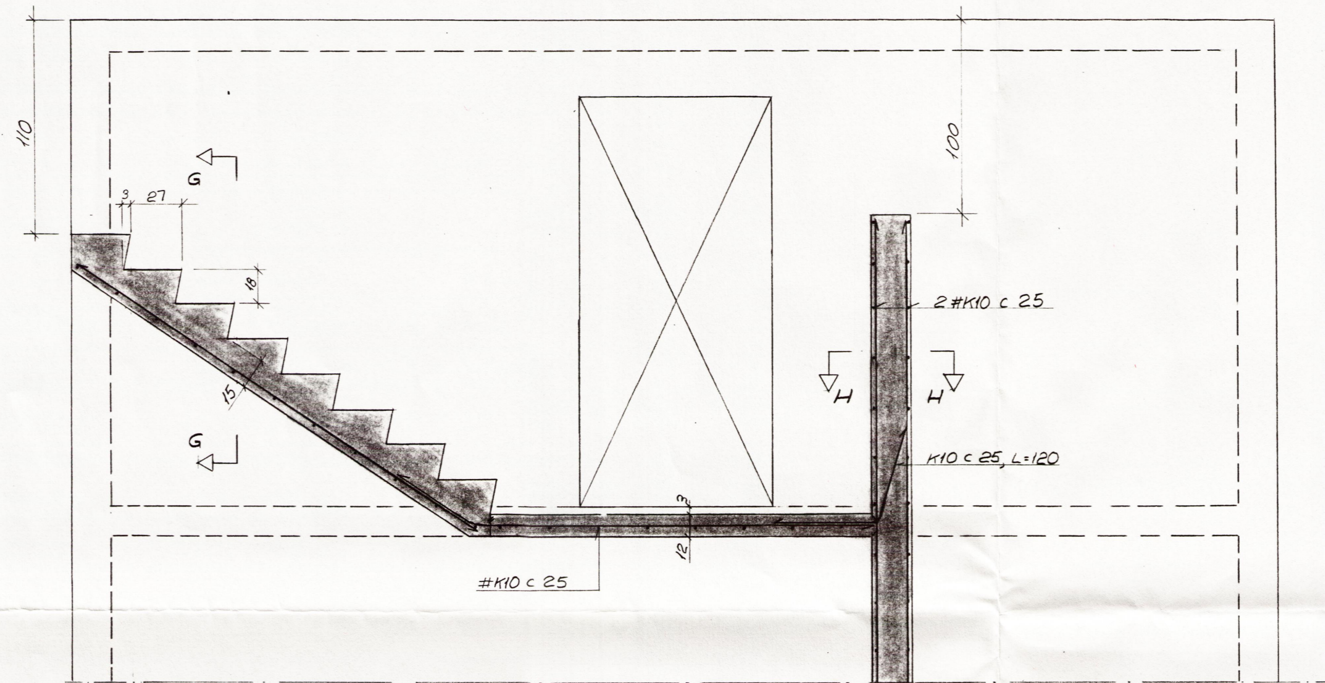
SNID F-F - 1:20
