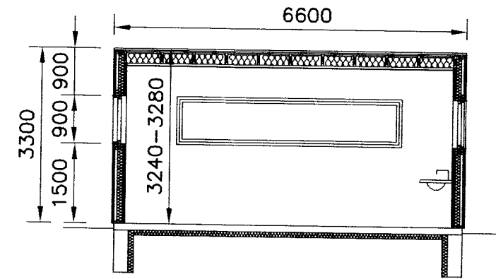
SNID 1:100
