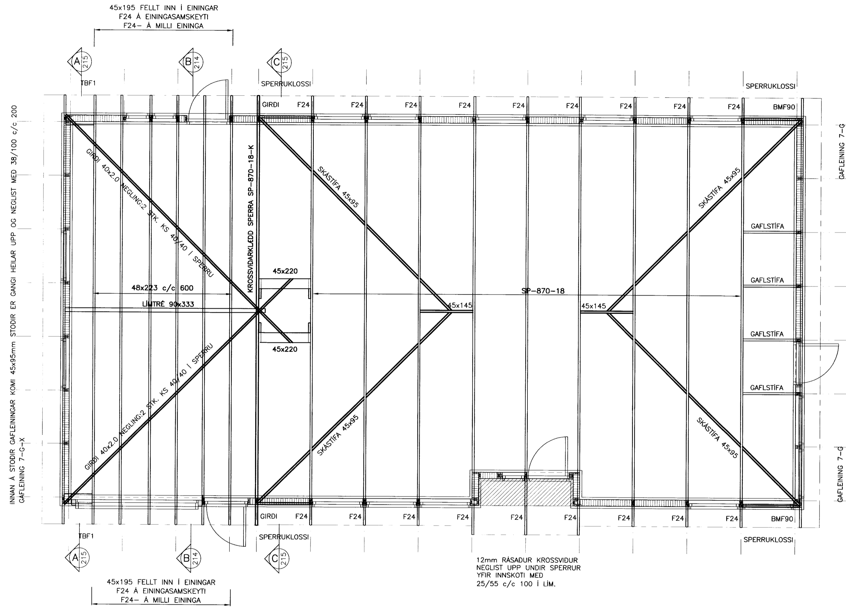
ÞAKPLAN MKV. 1:50
