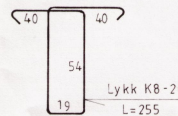
Snid B-B
