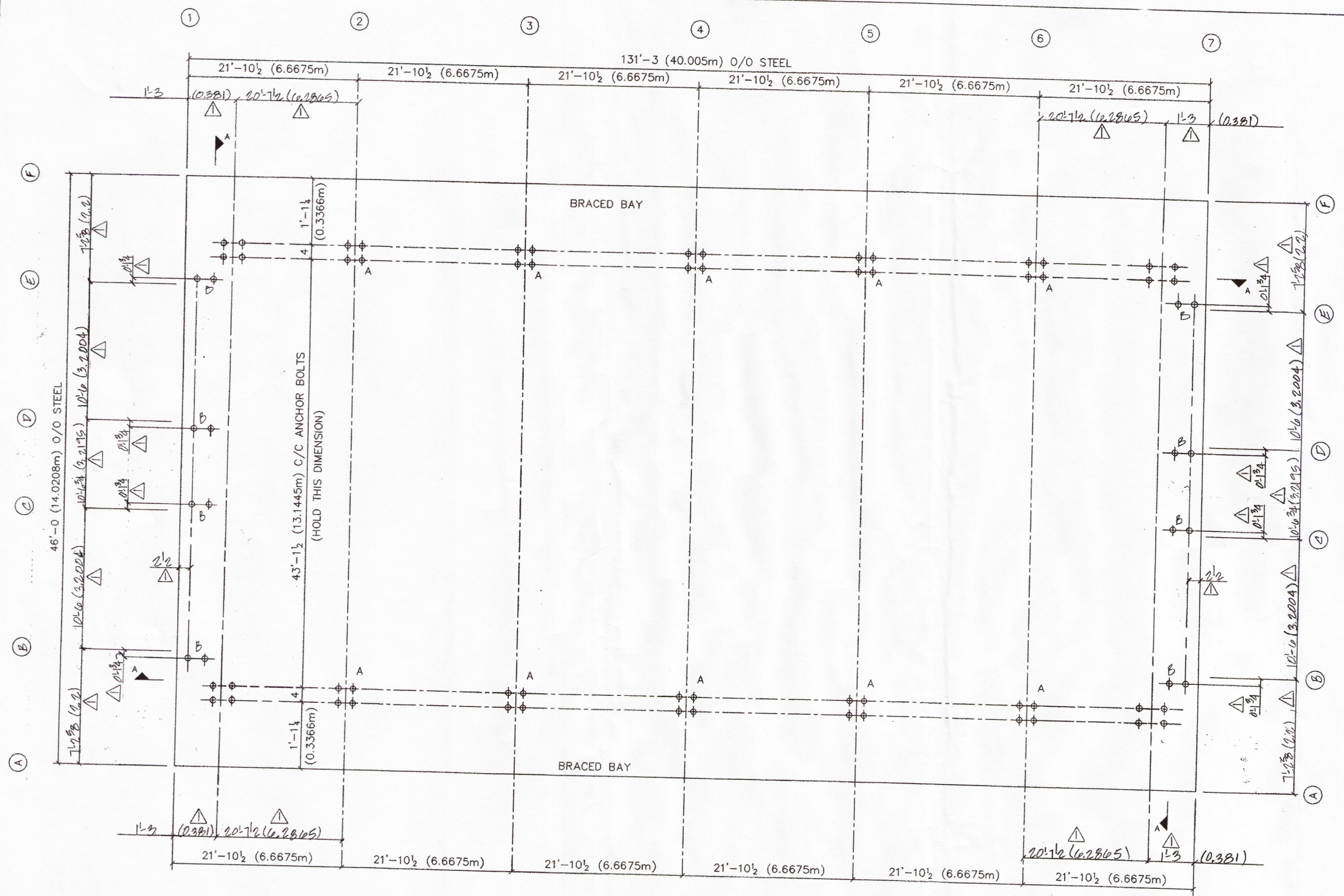
ANCHOR BOLT SETTING PLAN
