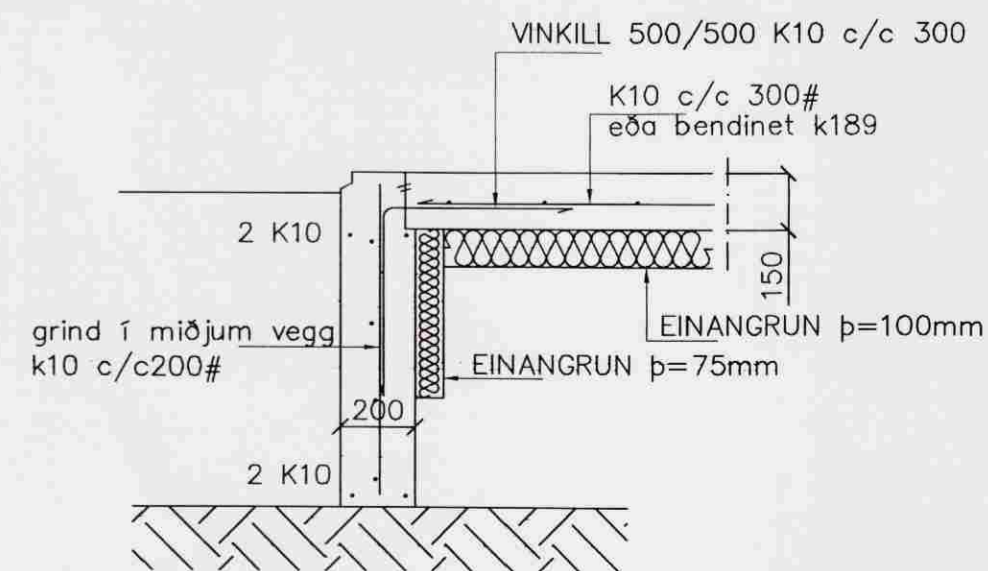
SNID 1 1:20
