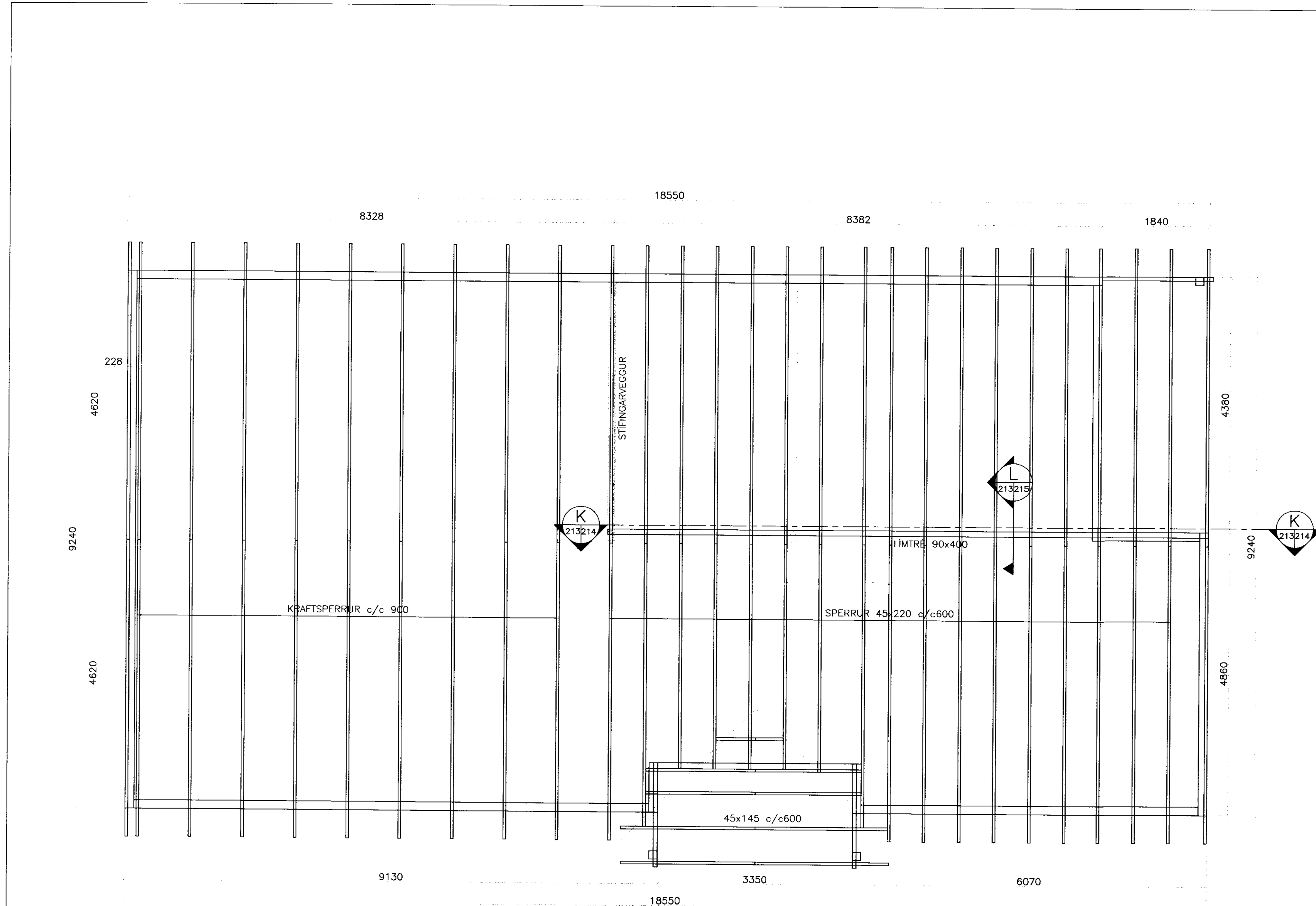
ÞAKPLAN
