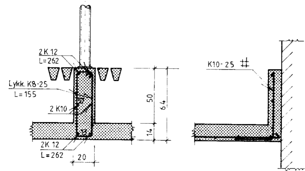
Snid B-B M=1:20
