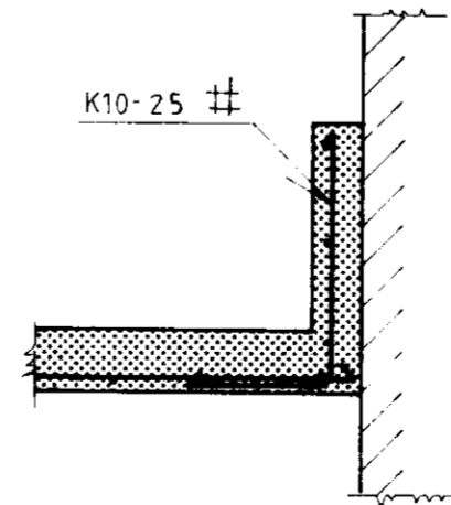
Snid B1-B1 M=1:20
