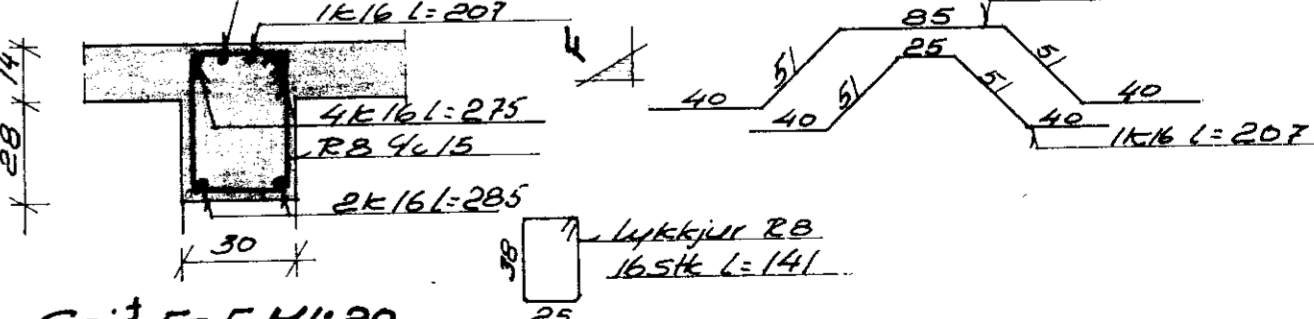
Snid F-F M1:20
