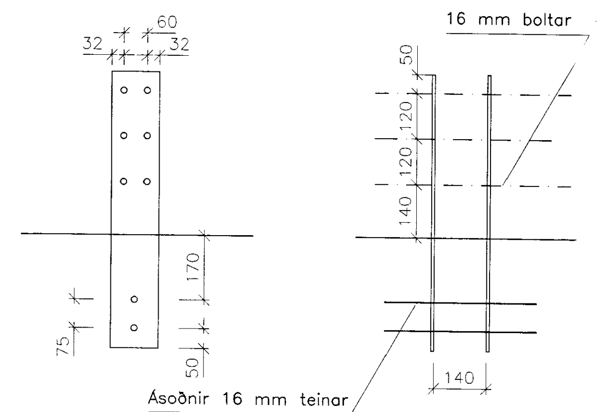
FESTING F3 1:10
