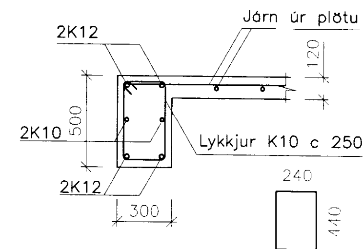
SNID A 1:20
