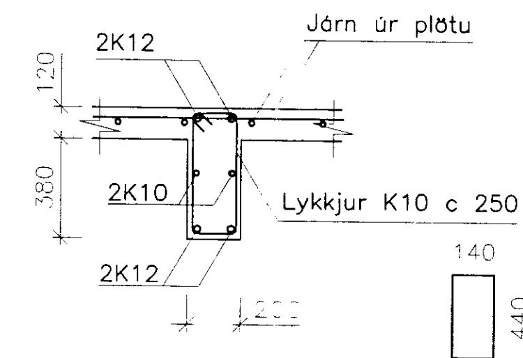
SNID B 1:20
