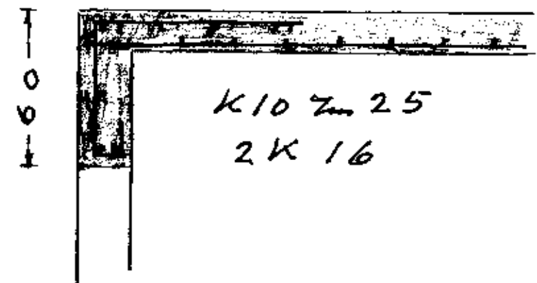
90 Sniff B-B 1:20
