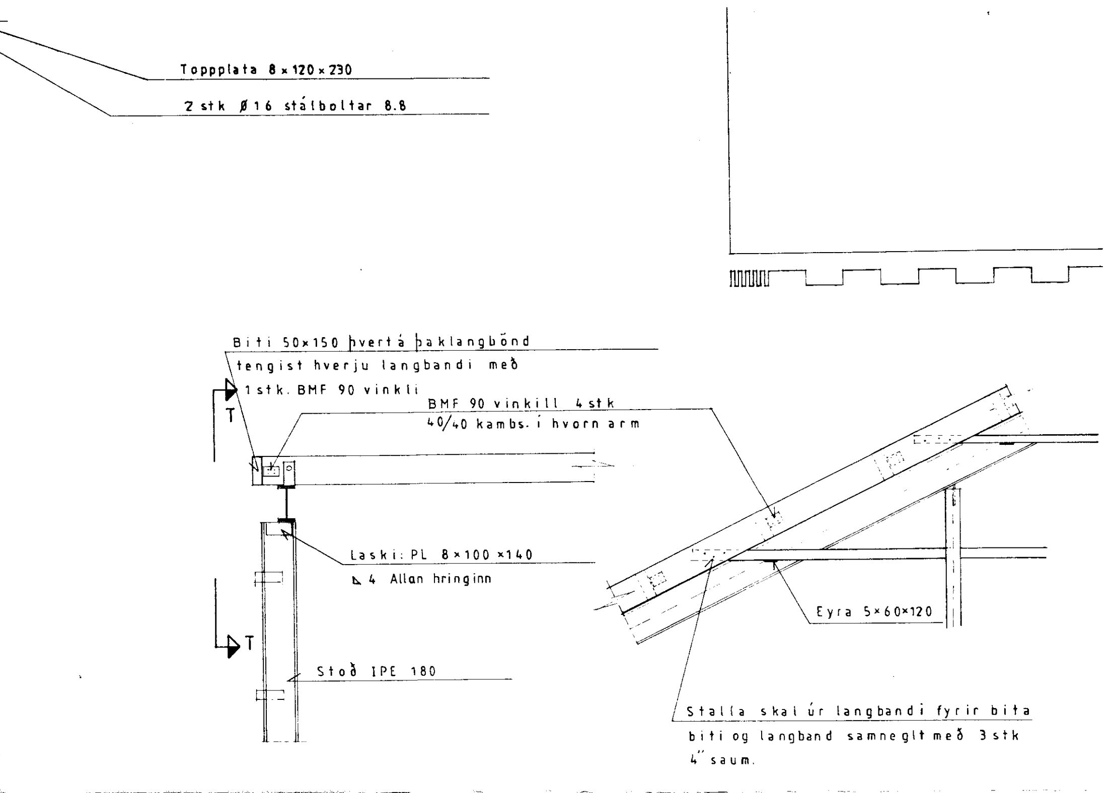
SNID S-S M=1:20
