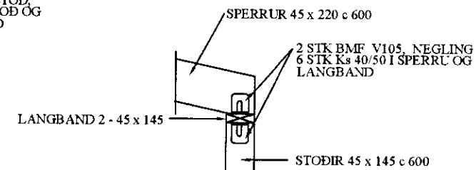
SNID C-C 1:20
