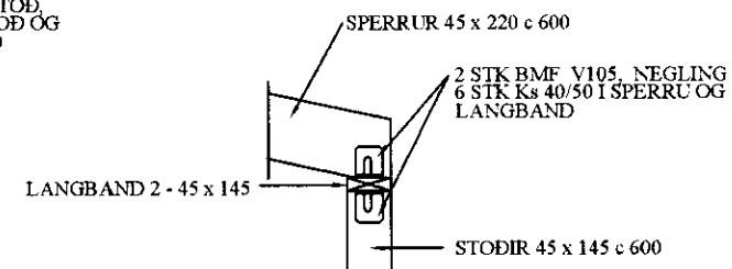
SNID C-C 1:20
