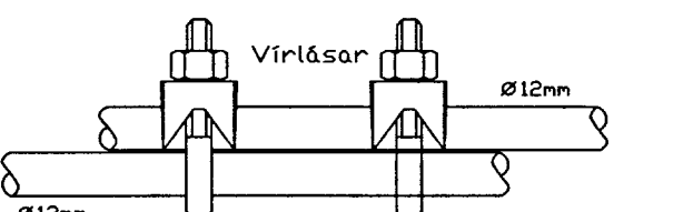
Santenging steyputeina
