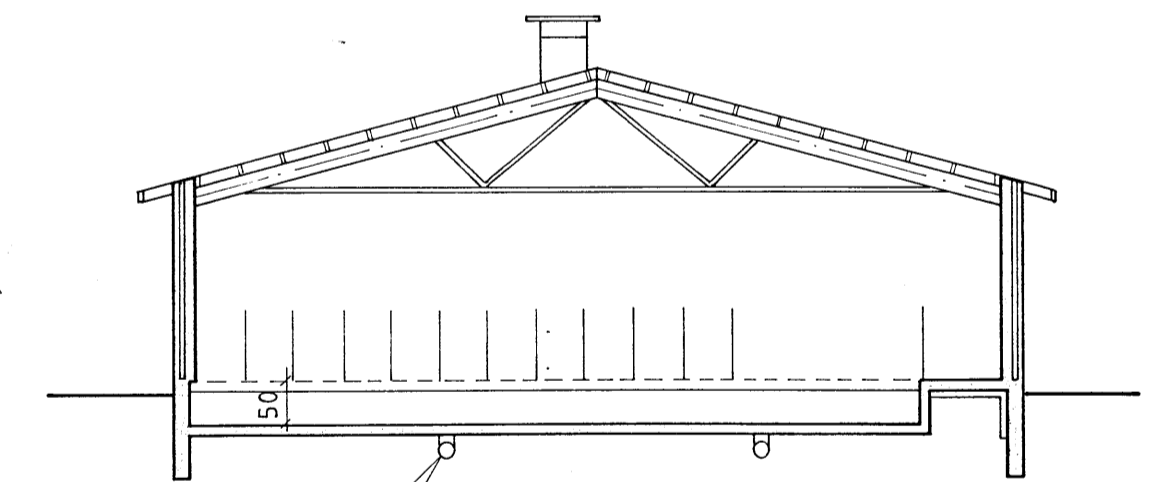
Snid B-B
