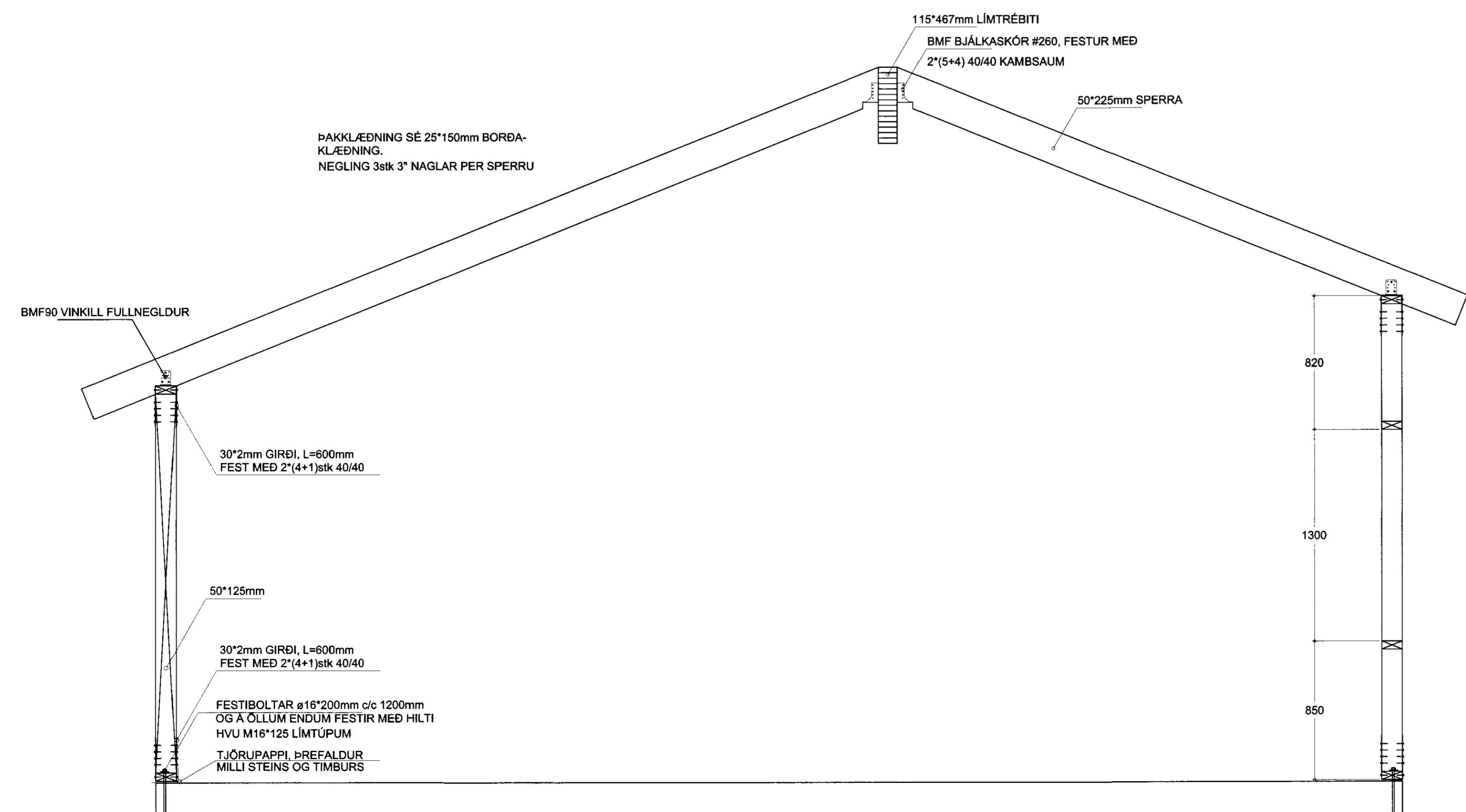
B SNEIÐING B, mkv. 1:20
