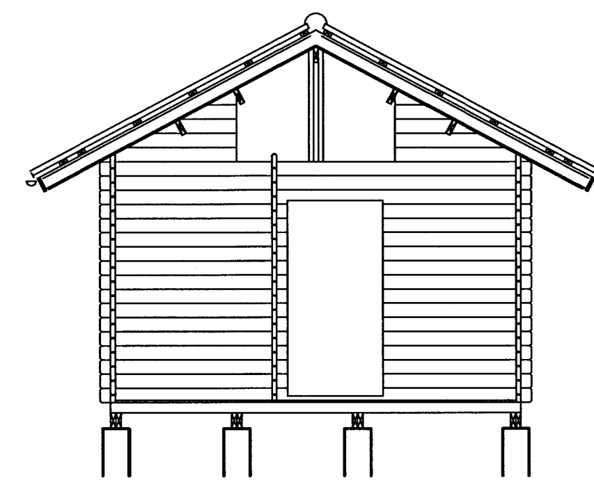
B SNID 1:50
